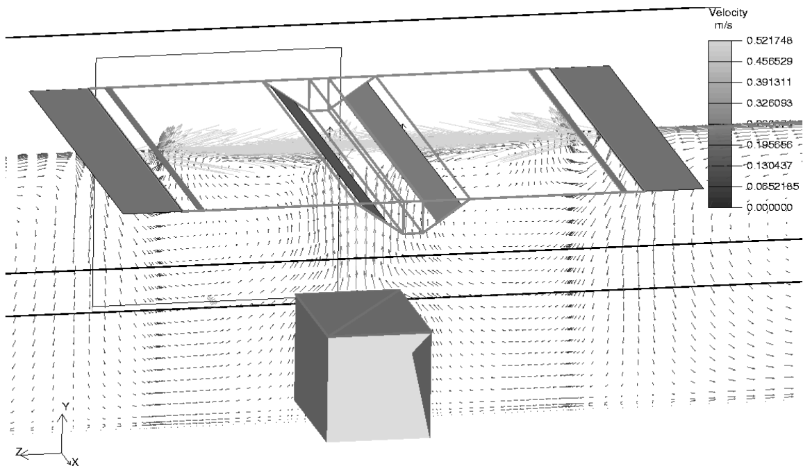
AirPak 2.0.6 Job: KCE43 (KCE system (supply 670 + 120 at 17.7 C / exhaust 840 l/s) with 5.6 kW appliance (vapour source 24.7 g/s)); version KCE4200
