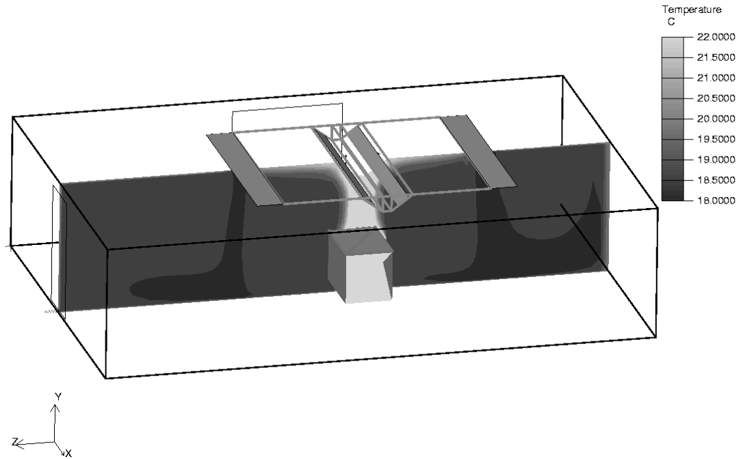
AirPak 2.0.6 Job: KCE4nc3 (KCE system with capture jets off (supply 790 at 17.7 C / exhaust 840 l/s) with 5.6 kW appliance (vapour source 24.7 g/s)); version KC
