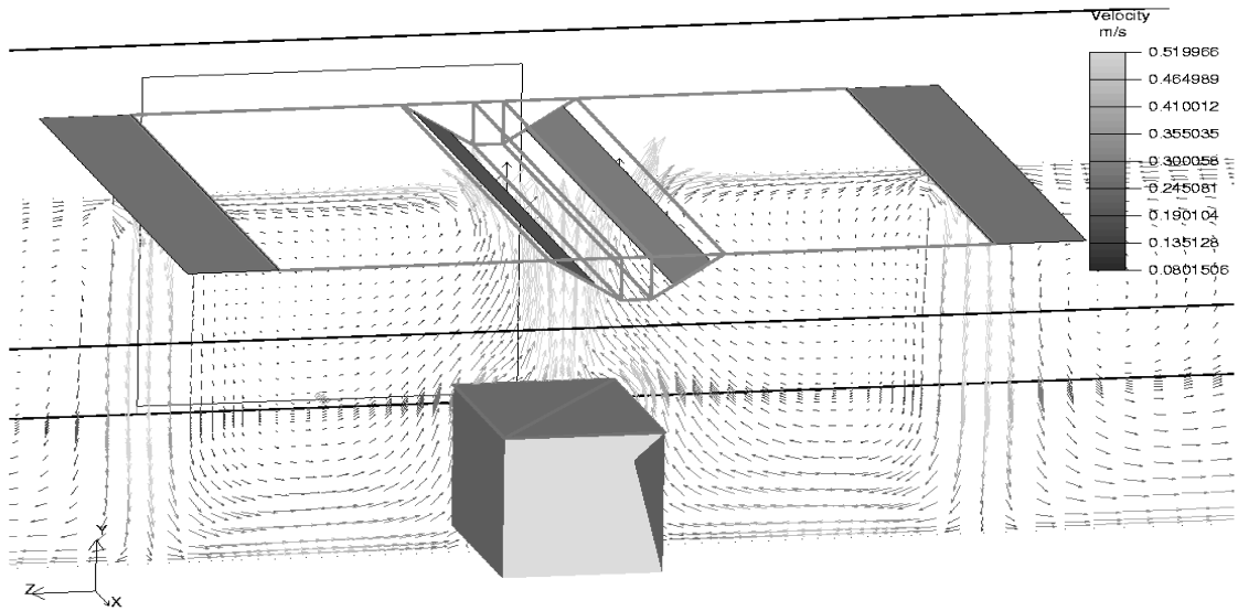
AirPak 2.0.6 Job: KCE4nc3 (KCE system with capture jets off (supply 790 at 17.7 C / exhaust 840 l/s) with 5.6 kW appliance (vapour source 24.7 g/s)); version KC
